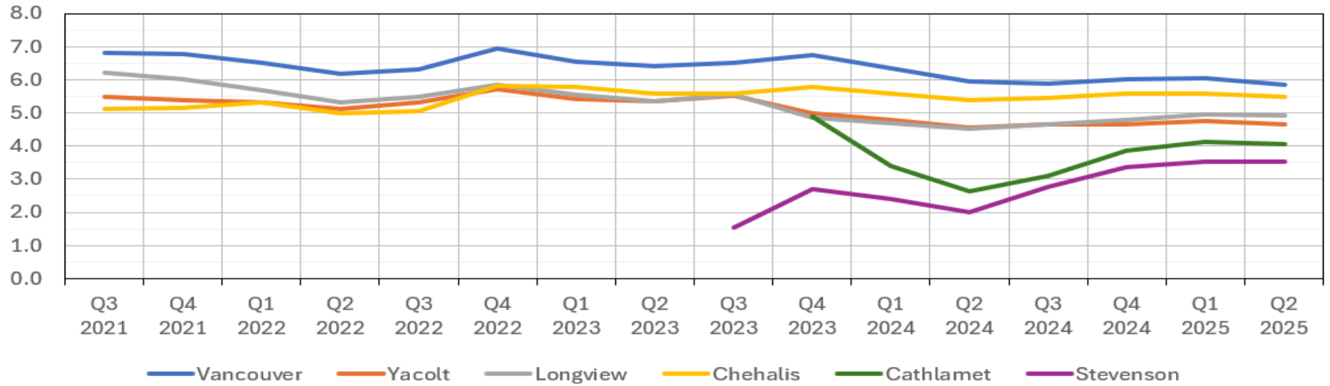
PM 2.5 - rolling annual averages - µg/m 3 [excluding flagged wildfire days] National Standard - 9 µg/m 3 (3-year annual average)
